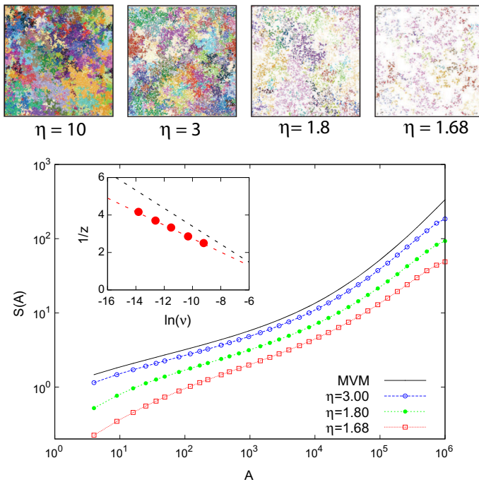
Fig. 10 (Top) Snapshots of configurations of the contact process with speciation at different values of the birth-to-death rate ratio \eta and \nu = 10^{-4} . In each panel, each color represents a different species. (Bottom) SARs at different values of the birth-to-death rate \eta (shown in the figure legend) and \nu = 10^{-5} . (Inset) Red dots: estimated exponent z as a function of \nu for the contact process with speciation at \eta = 1.68 . Red dashed line is a linear fit; black dashed line is the corresponding fit for the voter model with speciation for comparison. We have chosen a NN dispersal kernel in all panels (Color figure online)
