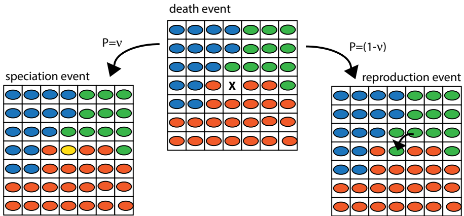
Fig. 1 Examples of transitions in the 2D voter model with speciation
