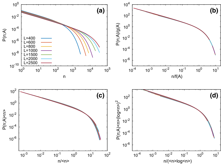
Fig. 5 SAD and data collapse. Results are presented for different linear system sizes and different speciation rates \nu , keeping the product A\nu = 200 constant. a SADs for different linear sizes from L = 400 to L = 2500 . b Collapse of SADs by means of Eqs. (13) and (16). The fitted parameter in the functions f and g is \epsilon = 0.08 . c Naive collapse without logarithmic corrections, where deviation for perfect collapse are evident. d Collapse with the scaling form of Eqs. (13) and (16), but setting \epsilon = 0 . Also in this case the discrepancy is evident
