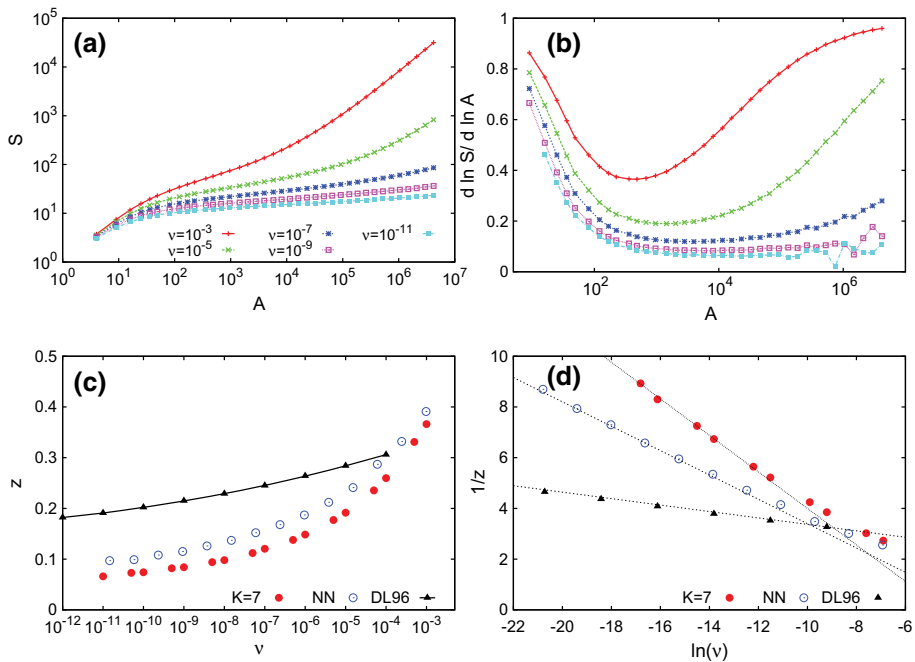
Fig. 3 Species–area relationships (SAR) and their scaling behavior in the voter model with speciation. a Number of species S as a function of the sampled area A for different speciation rates as in the caption. The triphasic shape is evident for larger speciations rates. Simulations from [77] were performed with a square dispersal kernel, i.e. P(\mathbf{r}) is a uniform distribution on a square of side K centered on the empty site, with K = 7 . b Local slopes, d \ln S / d \ln A for the curves shown in panel a . c Dependence of the exponent z on v as obtained from the local slopes for both the square kernel with K = 7 and NN dispersal. The exponent is estimated at the inflection point of the SADs, i.e. at the minimum of the local slopes. Also shown is the prediction of Eq. (8) (black solid line) where the black triangles correspond to the values provided in [31]. d Plot of 1/z versus \ln(v) of the same data of panel c to highlight the logarithmic behavior of Eq. (9)
