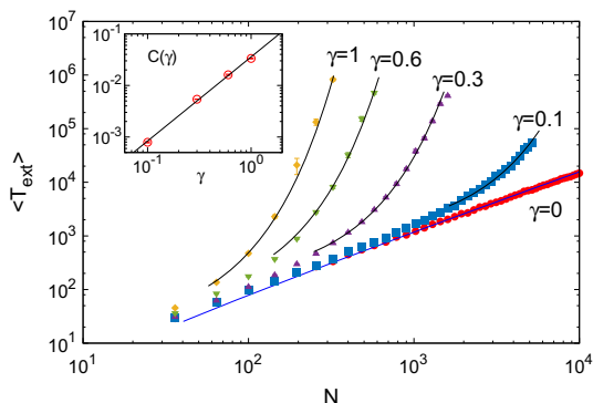
Fig. 11 Extinction times for the model with NN dispersal without immigration ( v = 0 ). Mean extinction time ( \langle T_{ext} \rangle ) as a function of N for different values of \gamma as in label. The blue curve approximating the neutral \gamma = 0 data points corresponds to the neutral expectation \langle T_{ext} \rangle \propto N \ln N , the black curves over the symbols for \gamma \neq 0 correspond to exponential fits of the form \langle T_{ext} \rangle \propto \exp(C(\gamma)N) . The inset shows (symbols) C(\gamma) versus \gamma , while the black solid line display the best fit C(\gamma) = A\gamma^\beta with \beta \approx 1.63 . The average extinction time is obtained by an annealed average, i.e. by randomizing the preference sites at each realization. Each point represents an average over 10^3 realizations
