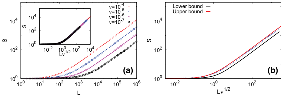
Fig. 4 Species–area relationships for the voter model in D = 1 . a Average number of species S versus the system size L for different \nu as labeled. Inset: same curves plotted vs L\sqrt{\nu} , notice the excellent collapse. b SAR for \nu = 10^{-5} compared with the theoretical upper (10) and lower (11) bounds
