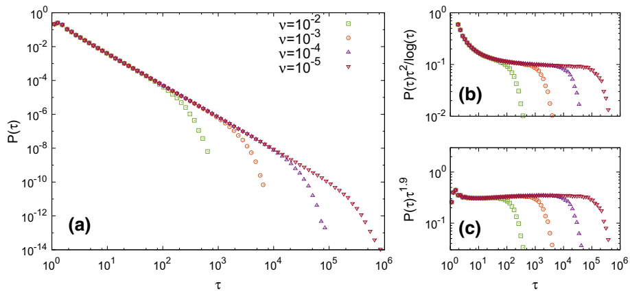
Fig. 8 Species persistence times. a Probability distribution function of species persistence times for different values of the speciation rate \nu as in label. Panels b and c show the pdf rescaled with the logarithmic correction, P(\tau)\tau^2/\ln \tau , and with a power law, P(\tau)\tau^{1.9} , respectively
