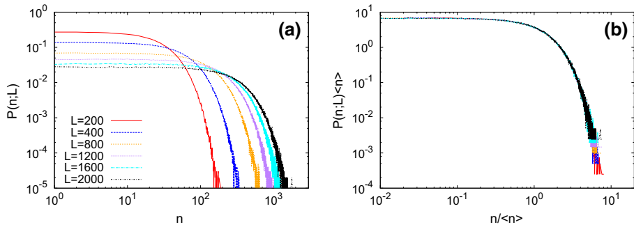
Fig. 7 Species abundance distribution (SAD) in the D = 1 voter model with speciation. a SAD P(n; L) versus n at varying the system size L as labelled with \Delta v = 40 constant. b Collapses of curves in a obtained with the rescaling SAD P(n; L) \langle n \rangle^{\nu} versus n / \langle n \rangle
