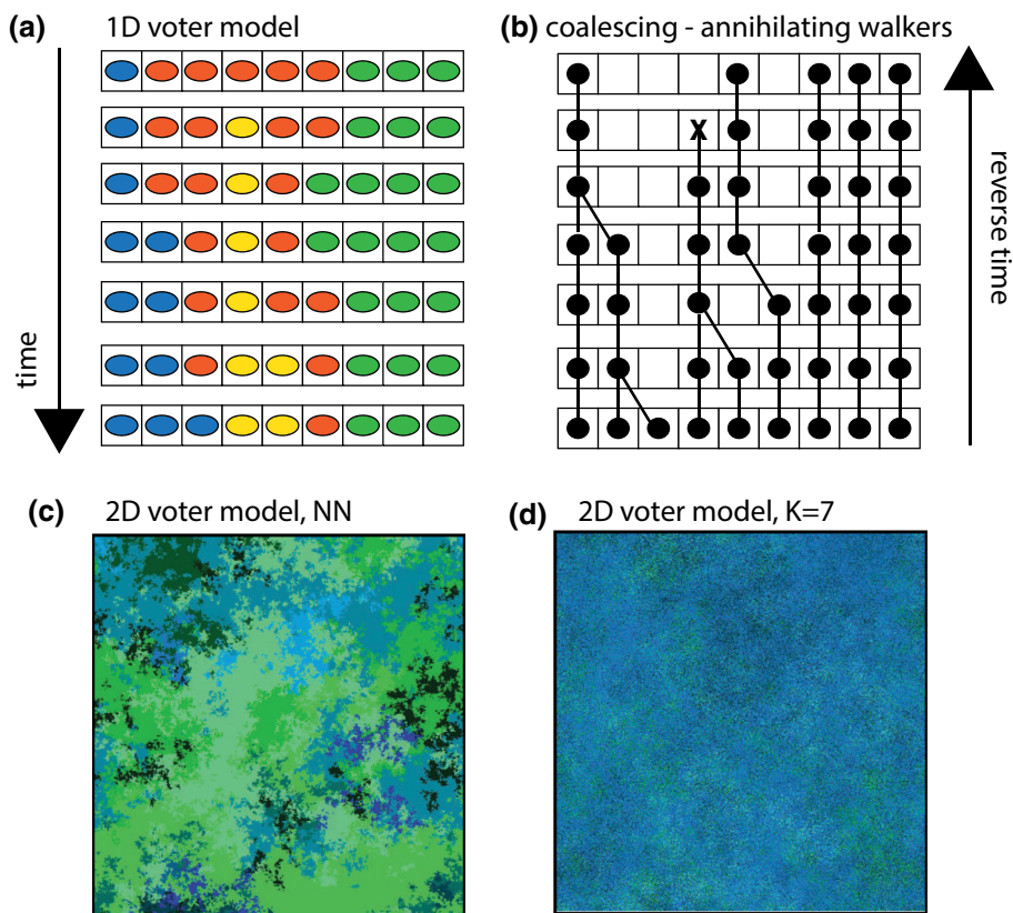
Fig. 2 a Example of space-time dynamics of the 1D voter model with speciation. b Corresponding dual dynamics: coalescing and annihilating random walkers. c Snapshot of a configuration of the 2D voter model simulated with the dual dynamics, with \nu = 5 \times 10^{-7} and nearest-neighbor (NN) dispersal. d Same as c but with a longer dispersal range (uniformly distributed in a square of side K ) with K = 7 . Each color labels a different species (Color figure online)
