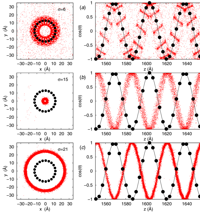
Figure 5. Two-dimensional projections (red dots) of the TF-bead trajectories of figure 4 for \sigma = 6 \text{ Å} (a), 15 \text{ Å} (b) and 21 \text{ Å} (c). Left panels refer to the projection onto the (x, y) -plane. Right panels show the cosine of the angle of rotation of the TF around the z -axis (DNA axis) as a function of the position along the z -axis itself. The black curves correspond to the DNA helix \cos(2\pi z/P) . Black full circles identify the DNA beads.
