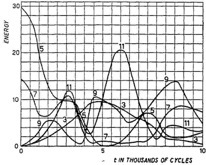
Fig. 5. - N = 32 ; \delta z^2 = 1/64 ; \beta = 1/16 . The initial configuration was a combination of 2 modes. The initial energy was chosen to be 2/3 in mode 5 and 1/3 in mode 7.
