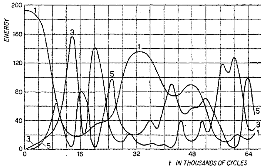
Fig. 6. - \delta z^2 = 2^{-6} . The force was taken as a broken linear function of displacement. The amplitude at which the slope changes was taken as 2^{-5} + 2^{-7} of the maximum amplitude. After this cut-off value, the force was assumed still linear but the slope increased by 25 percent. The effective N = 16 .
